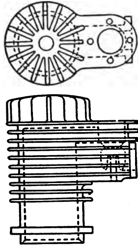
FIG. 6.—Air Cooled, Four Cycle Cylinder.
